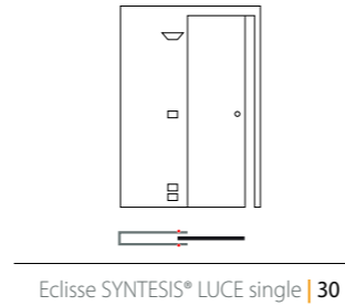
Eclisse SYNTESIS® LUCE single | 30
