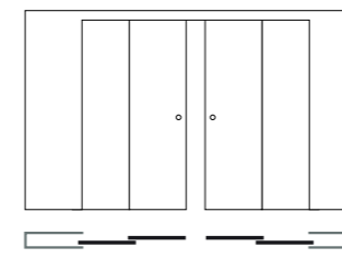
Eclisse TELESCOPIC double | 40
